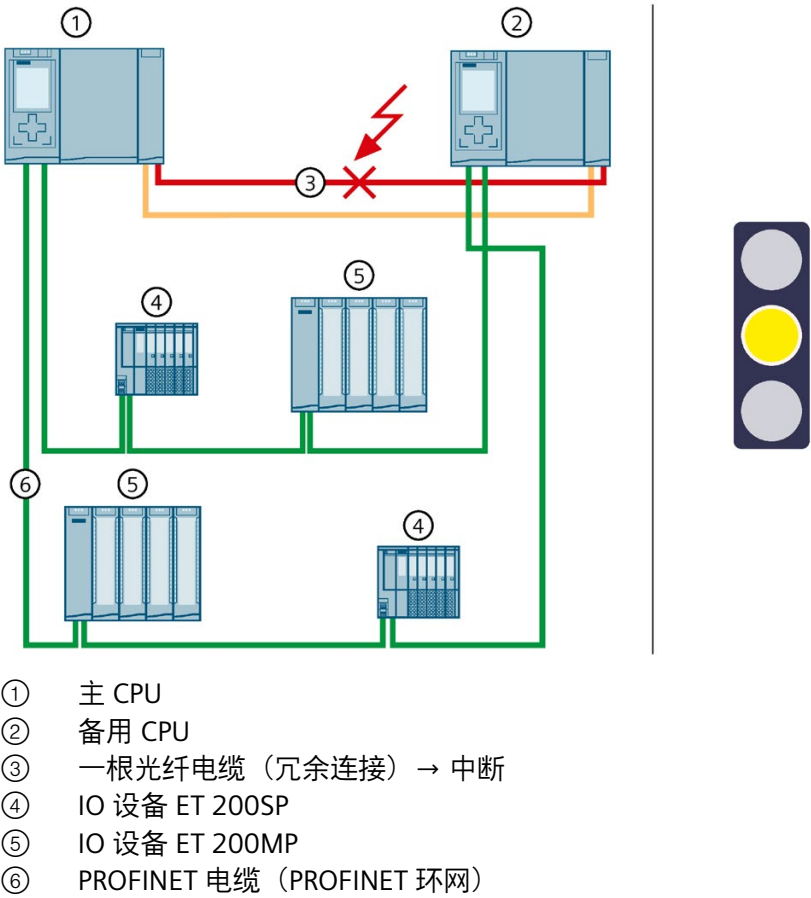
图 5-27 冗余连接故障
